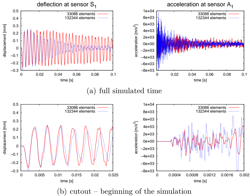
Figure 9: Two levels of discretization of the steel structure
